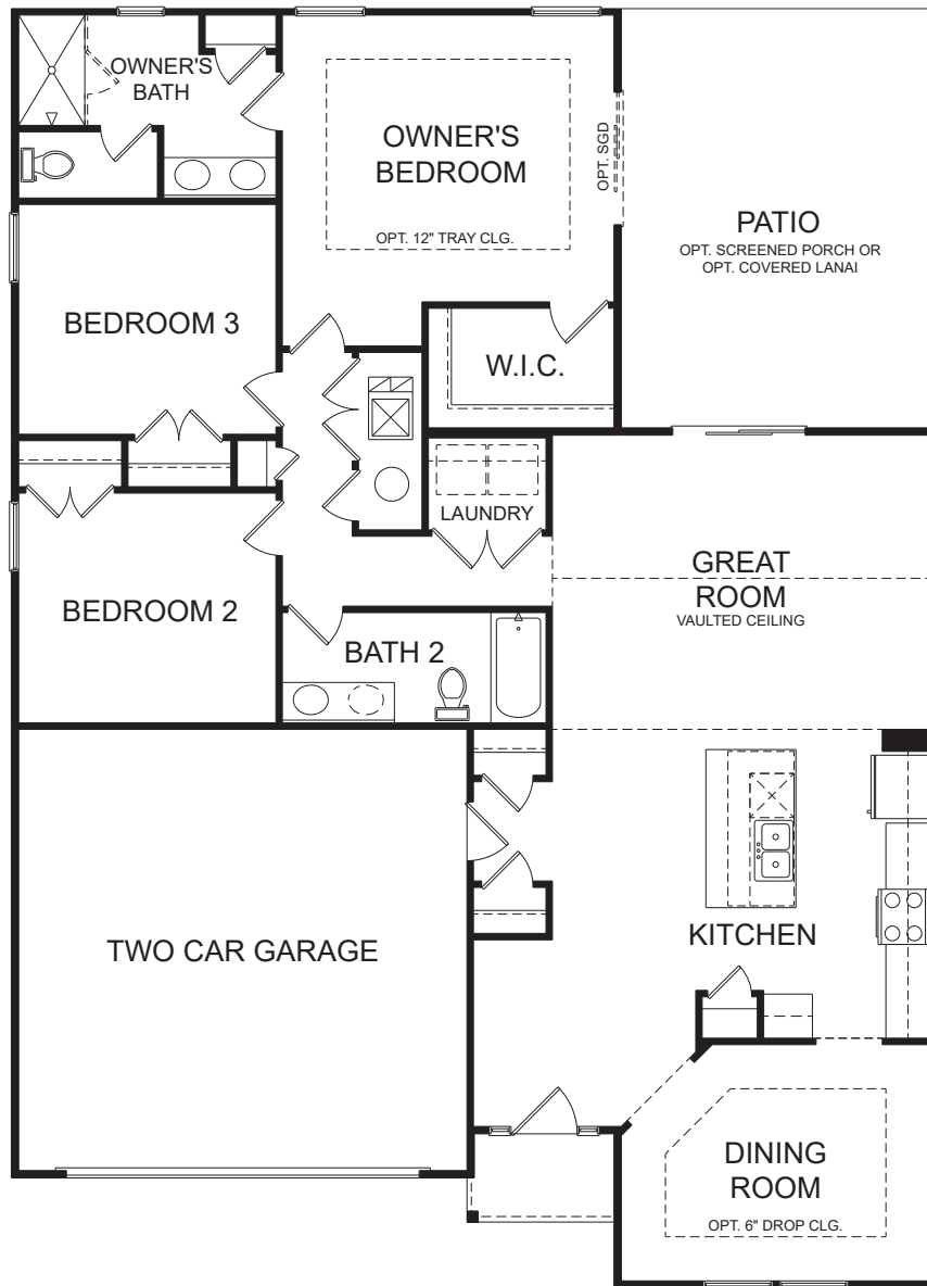
FLOOR PLAN
